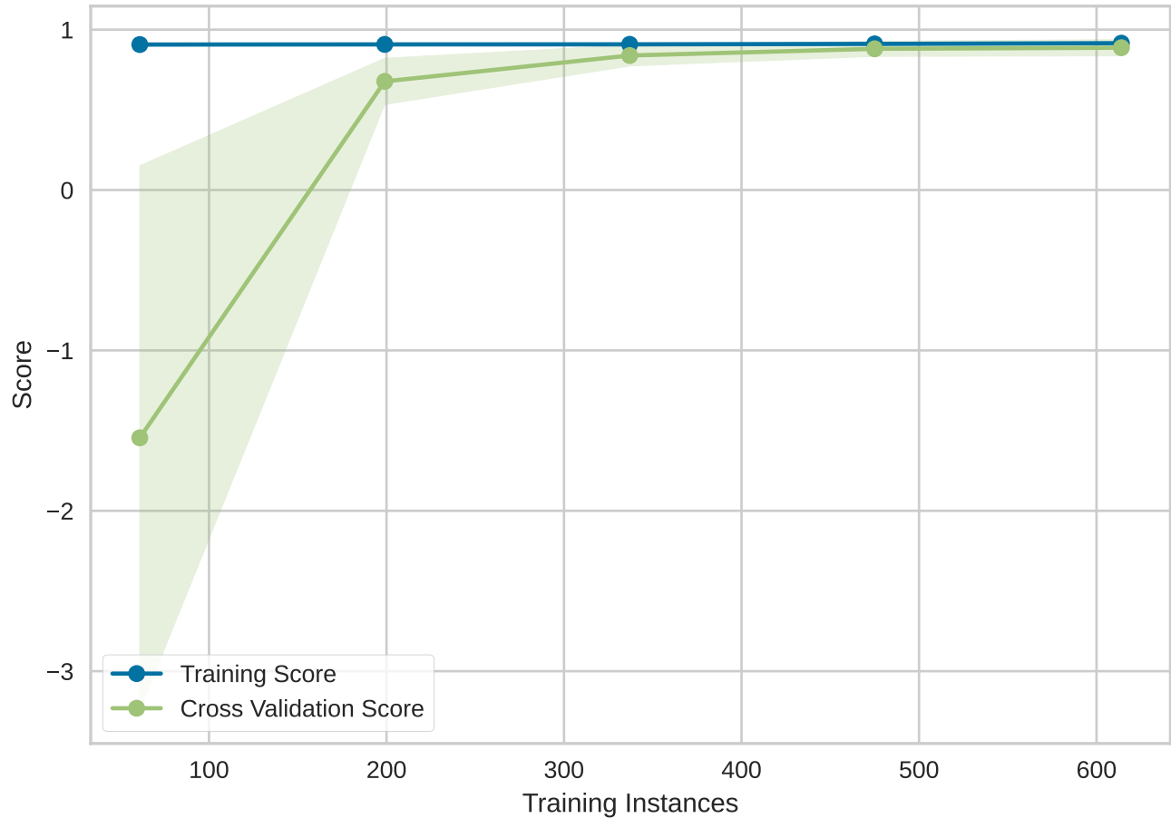
Learning Curve for RidgeCV
